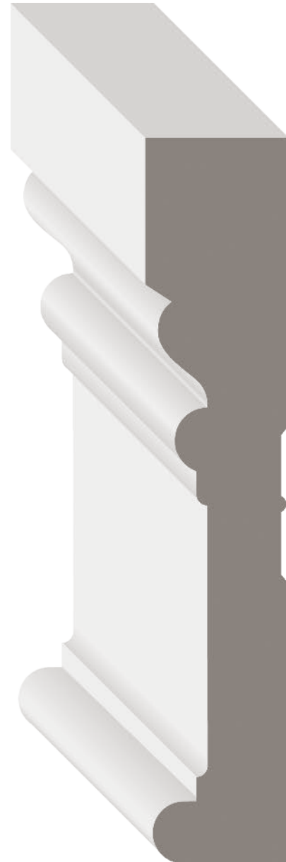
Stock Code Dimensions 190DHM 1 1/16" x 5 1/4" x 16' MDF/UL
