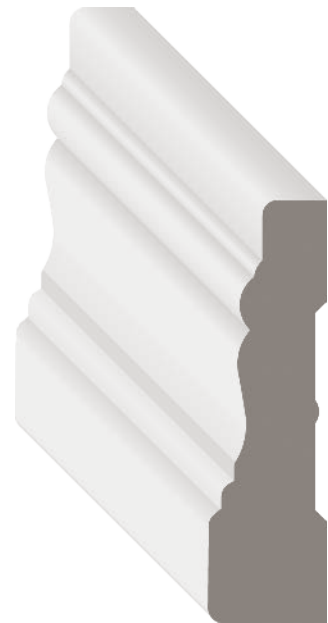
Stock Code Dimensions 347FJ \frac{5}{8} " x 2¼" x RL FJP
