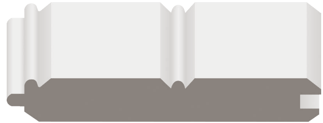
Stock Code: 3454TVGP Dimensions: 3/4" x 5 3/8" x 16' Material: FPP
