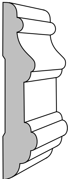
CHAIR RAIL F7410 9/16" X 3"
