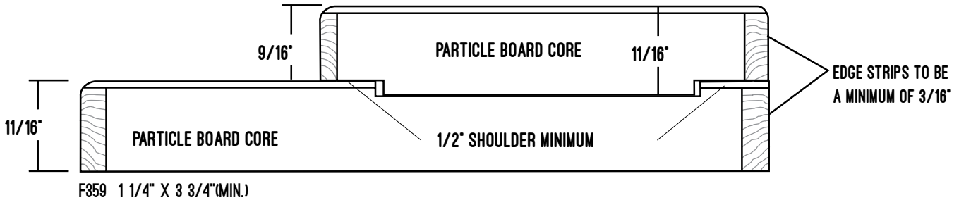
F359 1 1/4" X 3 3/4"(MIN.)
