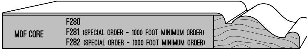
F280 - 5/8" X 5 1/4" F281 - 5/8" X 7 1/4" F282 - 5/8" X 9 1/4"
