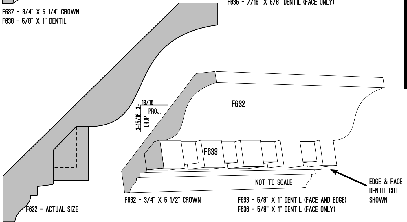
F630 - 3/4" X 3 1/2" CROWN F631 - 7/16" X 5/8" DENTIL (FACE AND EDGE) F635 - 7/16" X 5/8" DENTIL (FACE ONLY)
